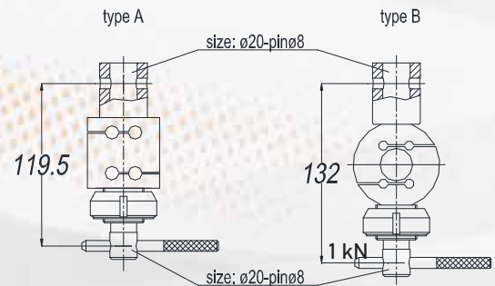
As auxiliary load cell (removable)
